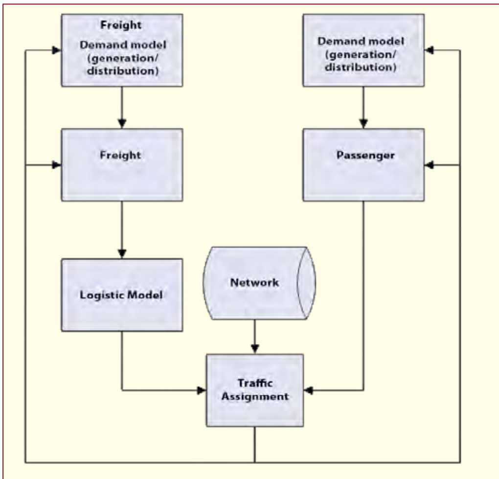
Figure 8: Trans-Tools structure
